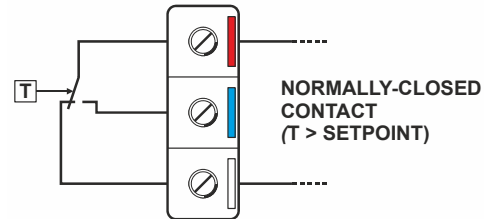
Fig. 2. Field wiring (frost protection)
