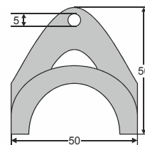
Fig. 3. Fastening clamp, dimensions in mm
